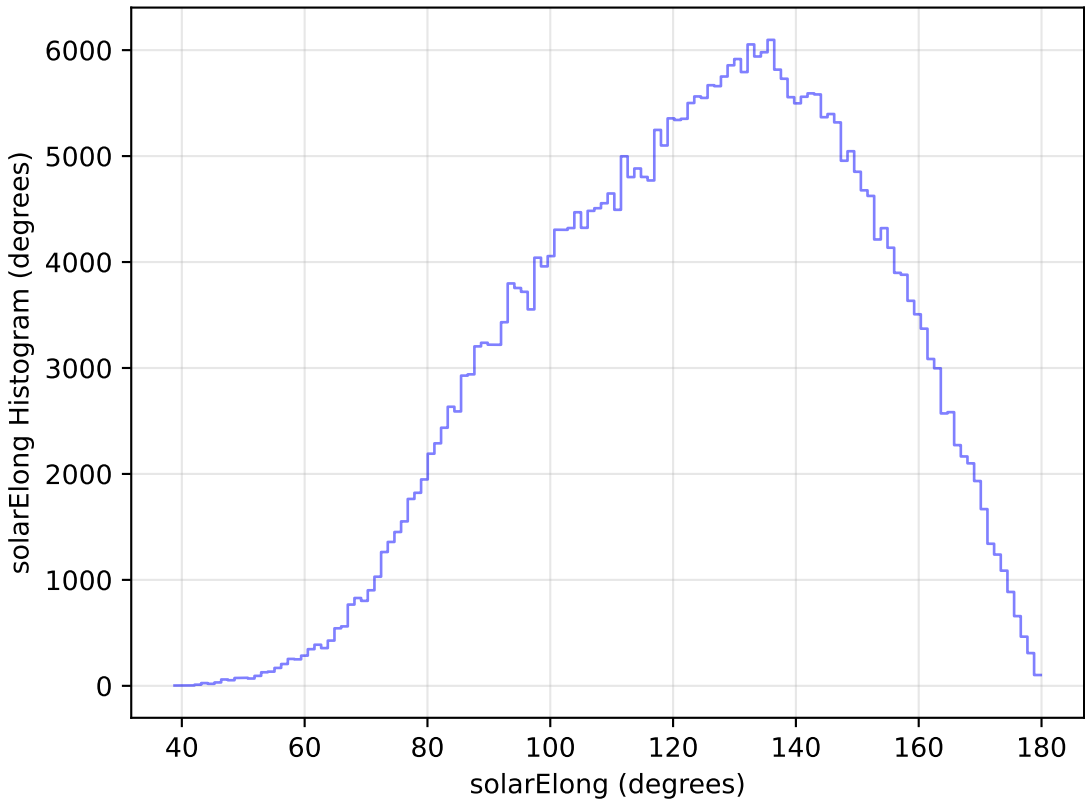
too_elab_r32_d3_giz_v3.4_10yrs All sky y band: solarElong Histogram
