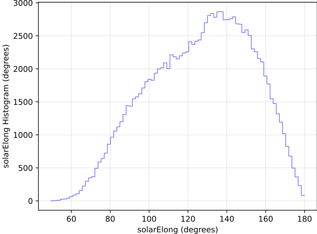
too_elab_r32_d3_giz_v3.4_10yrs All sky u band: solarElong Histogram
