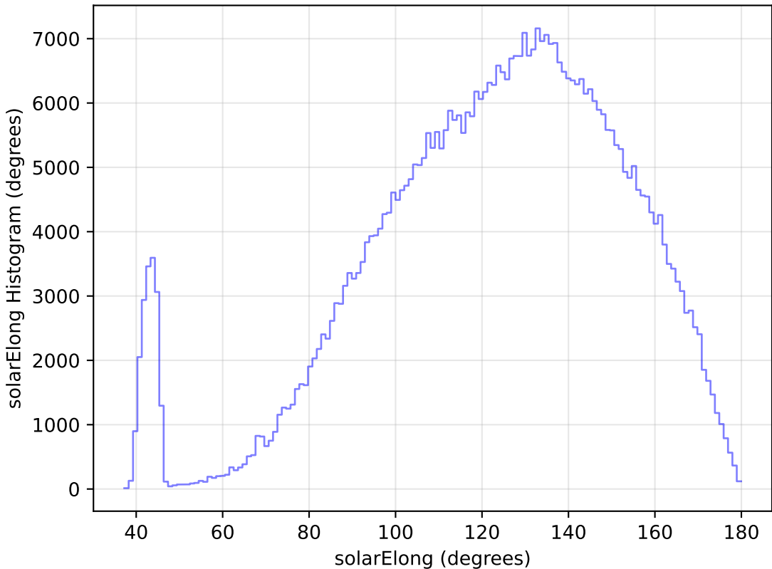
too_elab_r32_d3_giz_v3.4_10yrs All sky r band: solarElong Histogram
