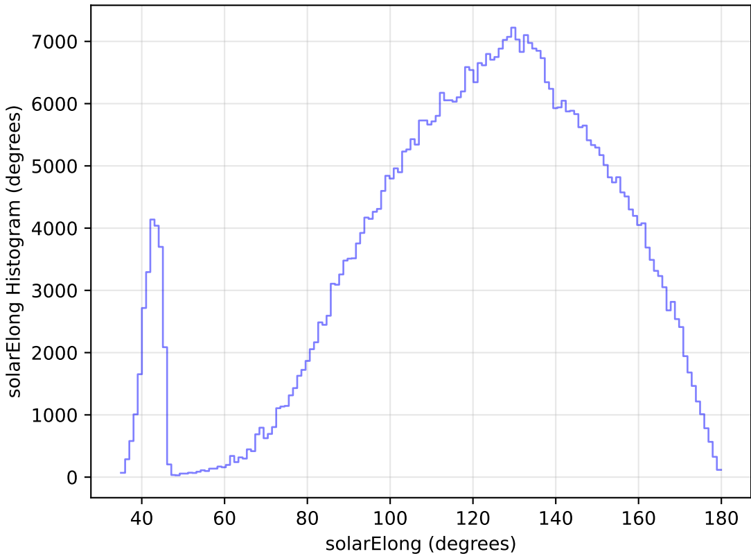
too_elab_r32_d3_giz_v3.4_10yrs All sky i band: solarElong Histogram
