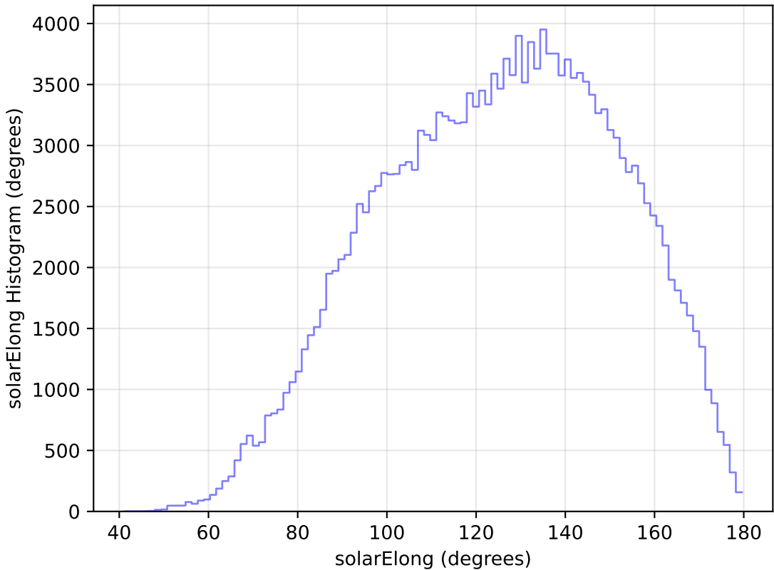
too_elab_r32_d3_giz_v3.4_10yrs All sky g band: solarElong Histogram
