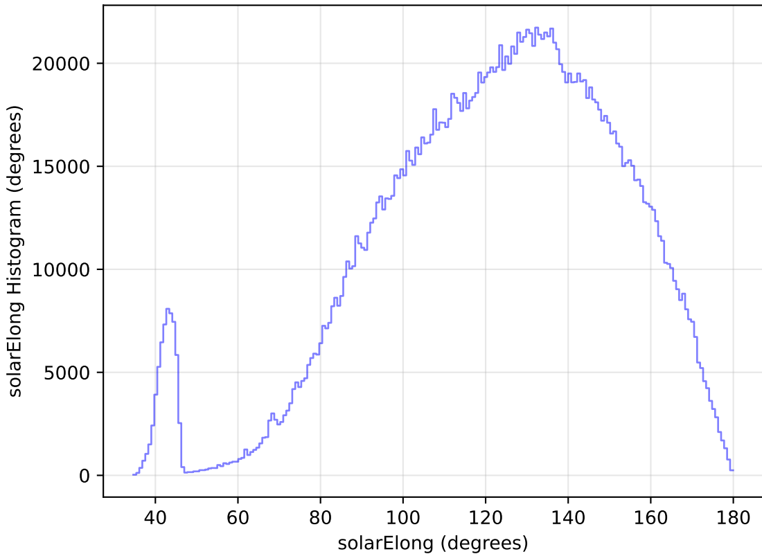
too_elab_r32_d3_giz_v3.4_10yrs All sky all bands: solarElong Histogram
