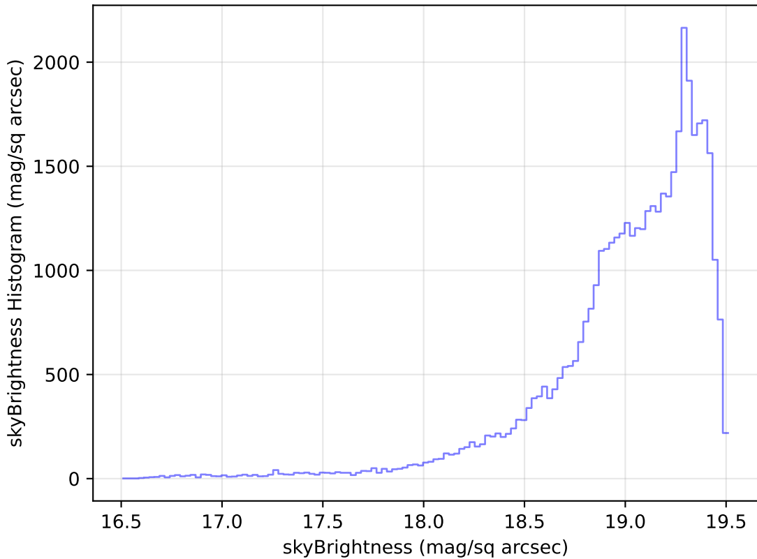
too_elab_r32_d3_giz_v3.4_10yrs Yr 1 z band: skyBrightness Histogram
