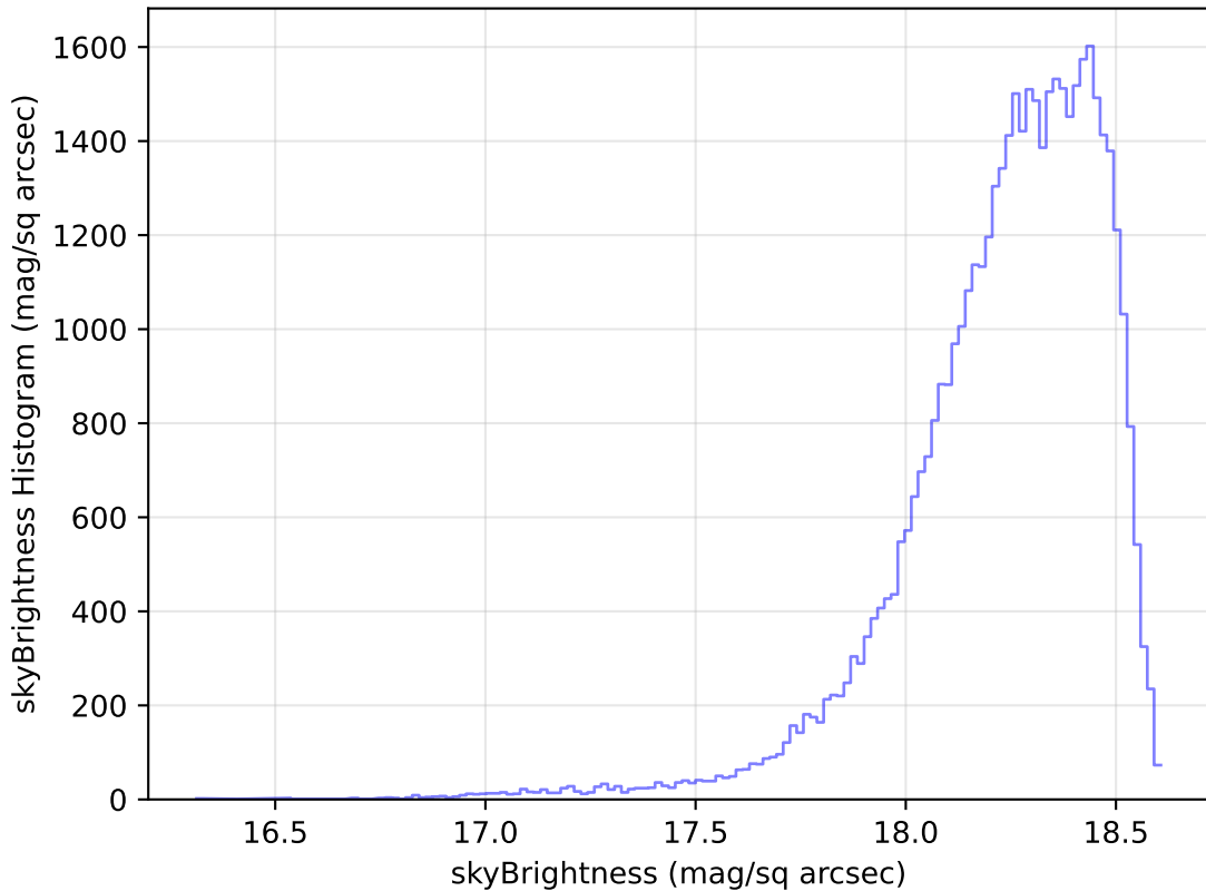
too_elab_r32_d3_giz_v3.4_10yrs Yr 1 y band: skyBrightness Histogram
