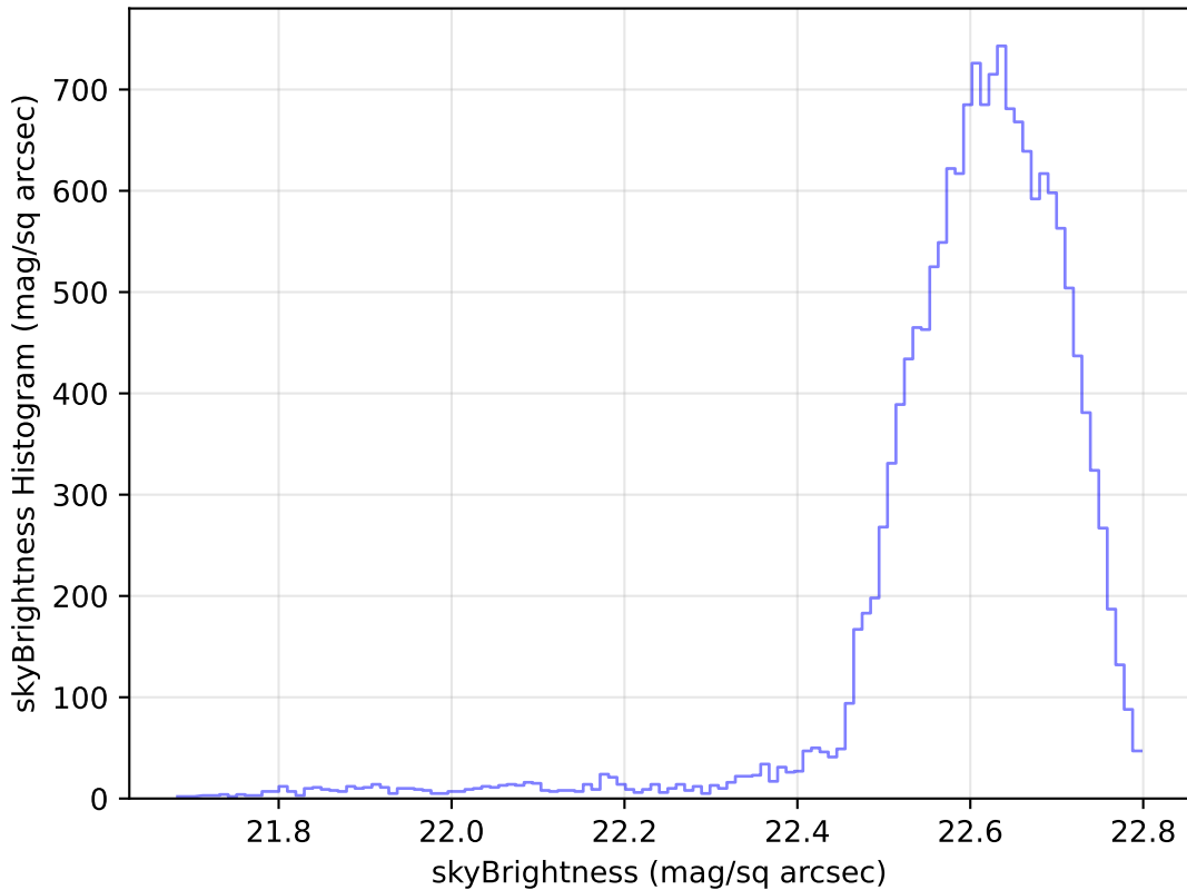
too_elab_r32_d3_giz_v3.4_10yrs Yr 1 u band: skyBrightness Histogram
