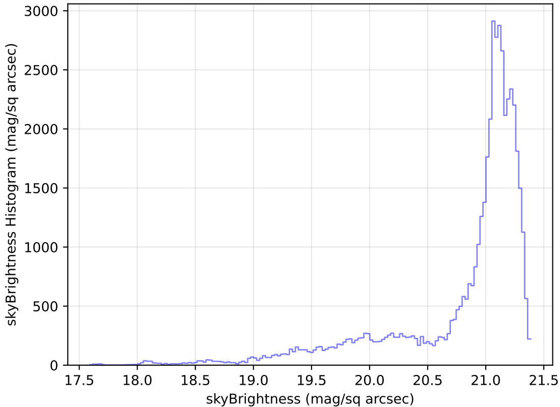
too_elab_r32_d3_giz_v3.4_10yrs Yr 1 r band: skyBrightness Histogram
