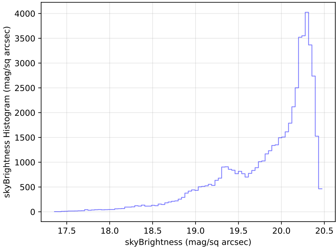
too_elab_r32_d3_giz_v3.4_10yrs Yr 1 i band: skyBrightness Histogram
