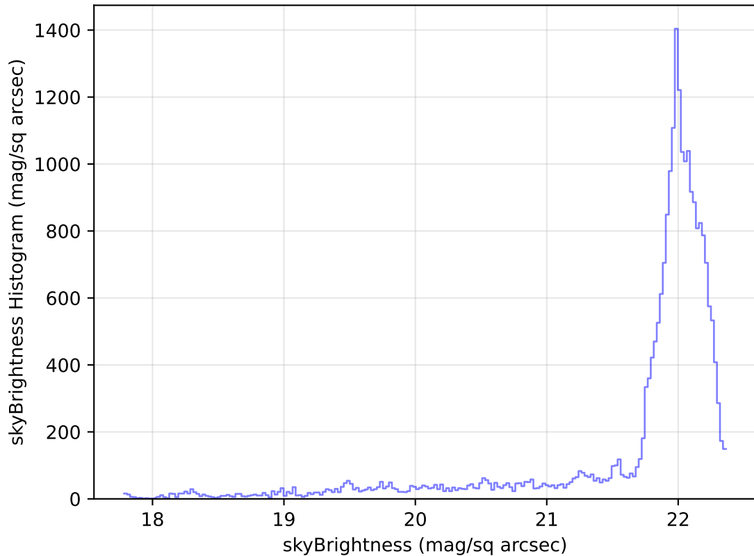
too_elab_r32_d3_giz_v3.4_10yrs Yr 1 g band: skyBrightness Histogram
