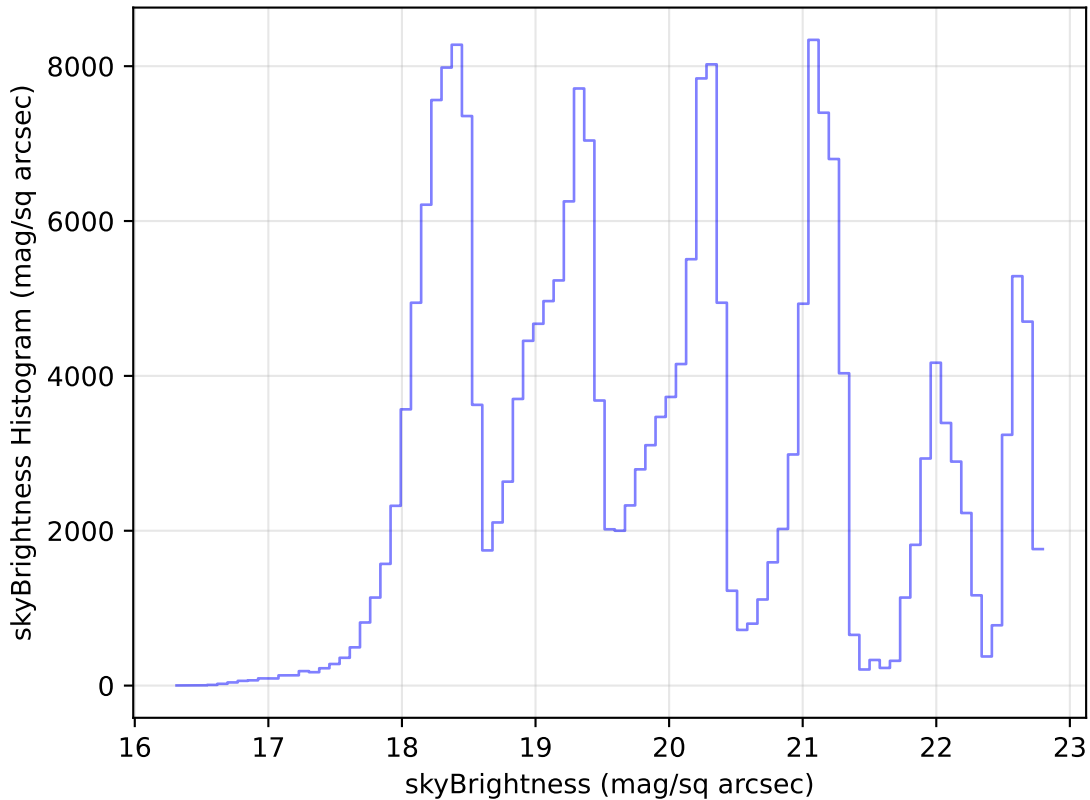
too_elab_r32_d3_giz_v3.4_10yrs Yr 1 all bands: skyBrightness Histogram
