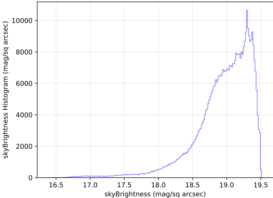
too_elab_r32_d3_giz_v3.4_10yrs WFD z band: skyBrightness Histogram
