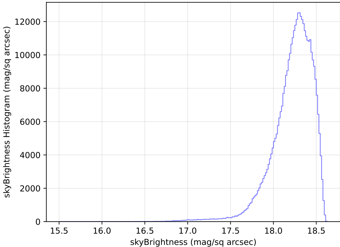
too_elab_r32_d3_giz_v3.4_10yrs WFD y band: skyBrightness Histogram
