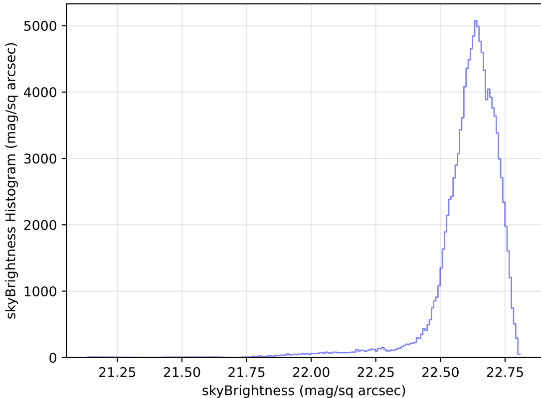
too_elab_r32_d3_giz_v3.4_10yrs WFD u band: skyBrightness Histogram
