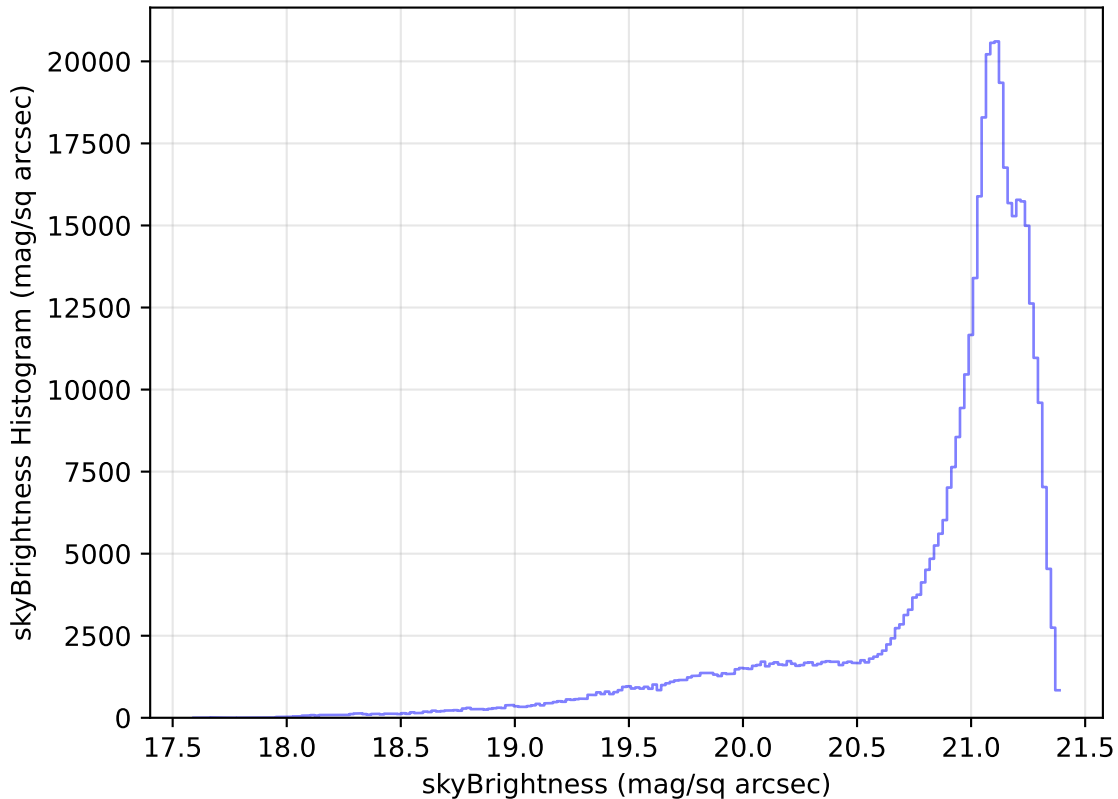
too_elab_r32_d3_giz_v3.4_10yrs WFD r band: skyBrightness Histogram
