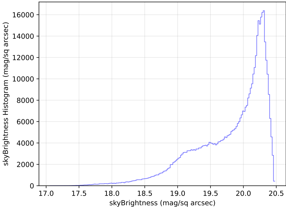
too_elab_r32_d3_giz_v3.4_10yrs WFD i band: skyBrightness Histogram
