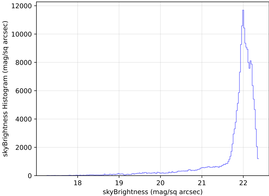
too_elab_r32_d3_giz_v3.4_10yrs WFD g band: skyBrightness Histogram
