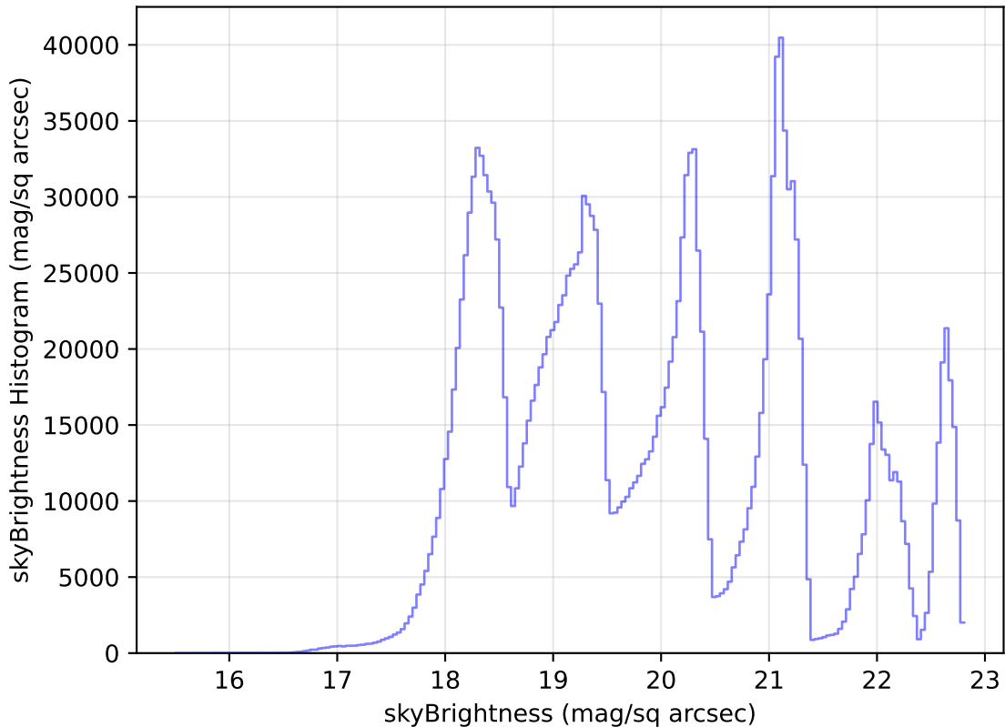
too_elab_r32_d3_giz_v3.4_10yrs WFD all bands: skyBrightness Histogram
