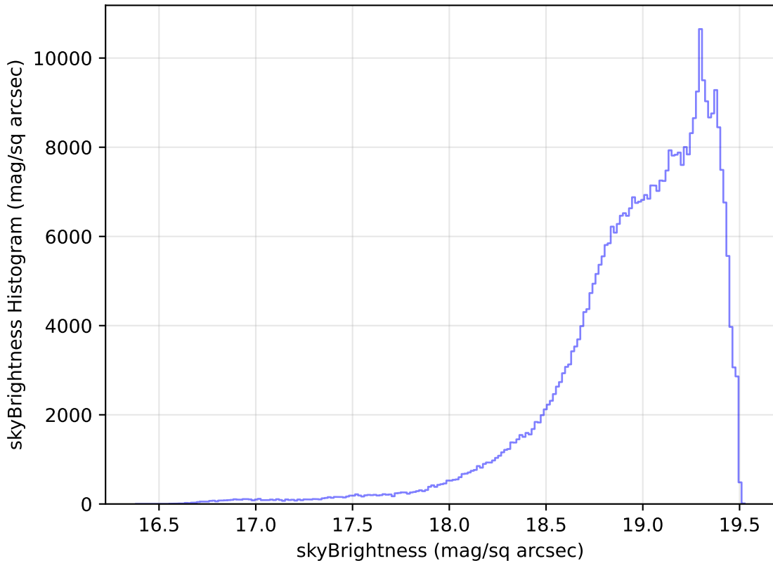
too_elab_r32_d3_giz_v3.4_10yrs All sky z band: skyBrightness Histogram
