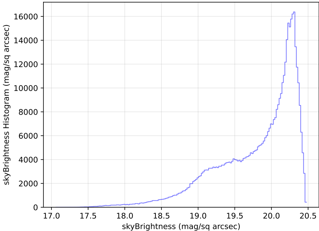
too_elab_r32_d3_giz_v3.4_10yrs All sky i band: skyBrightness Histogram
