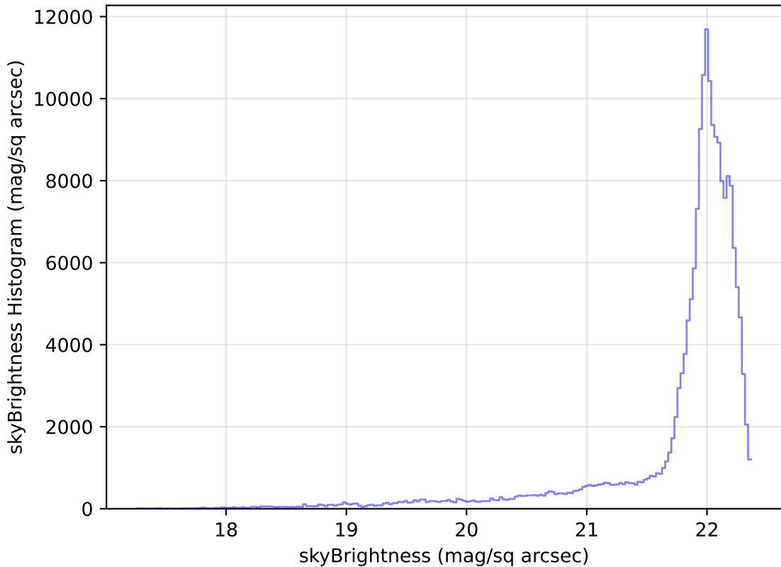
too_elab_r32_d3_giz_v3.4_10yrs All sky g band: skyBrightness Histogram
