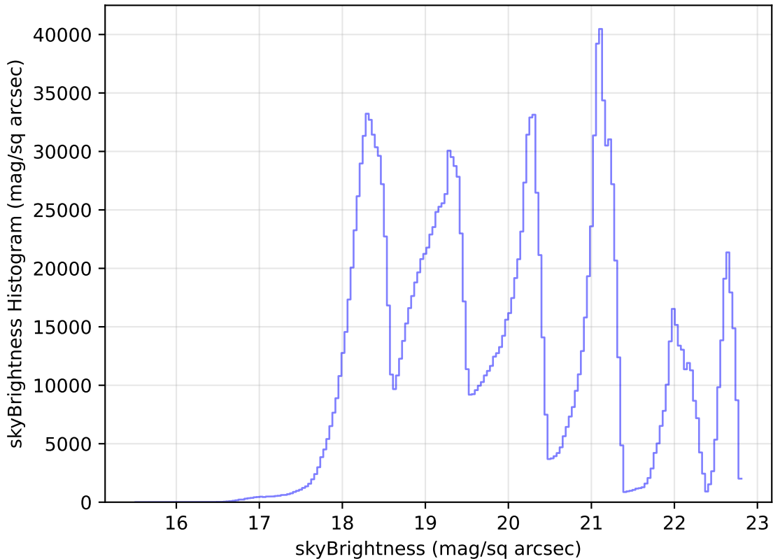
too_elab_r32_d3_giz_v3.4_10yrs All sky all bands: skyBrightness Histogram
