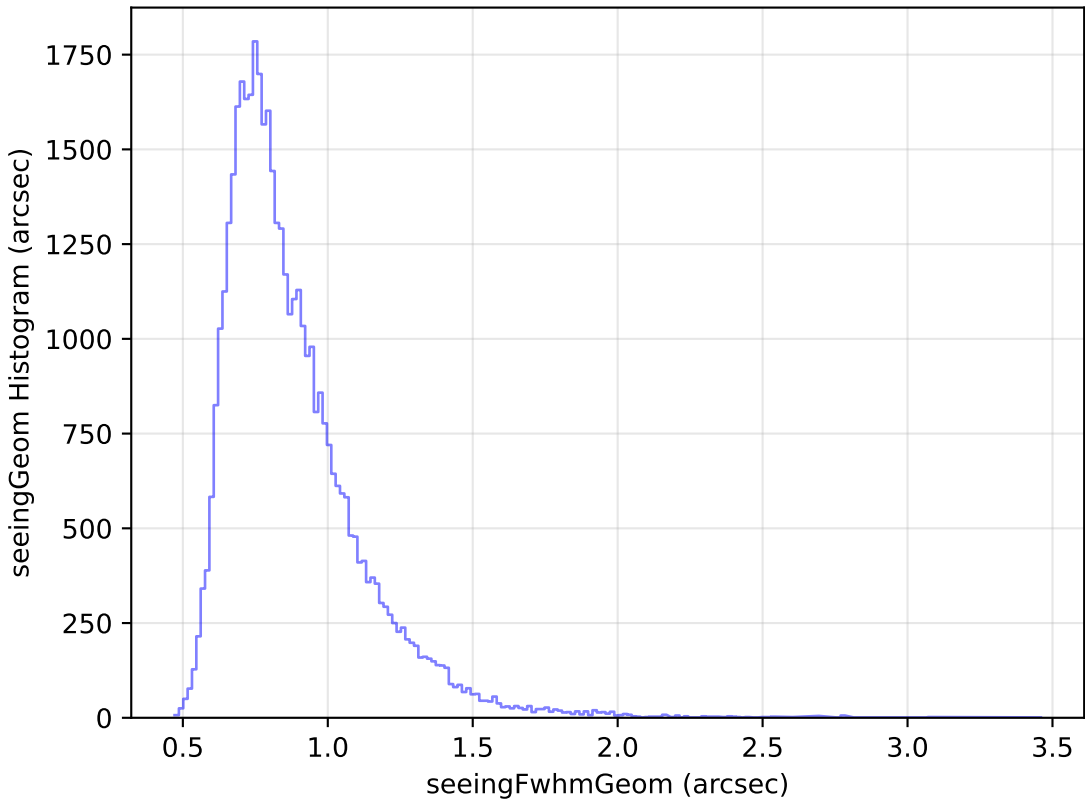
too_elab_r32_d3_giz_v3.4_10yrs Yr 1 z band: seeingGeom Histogram
