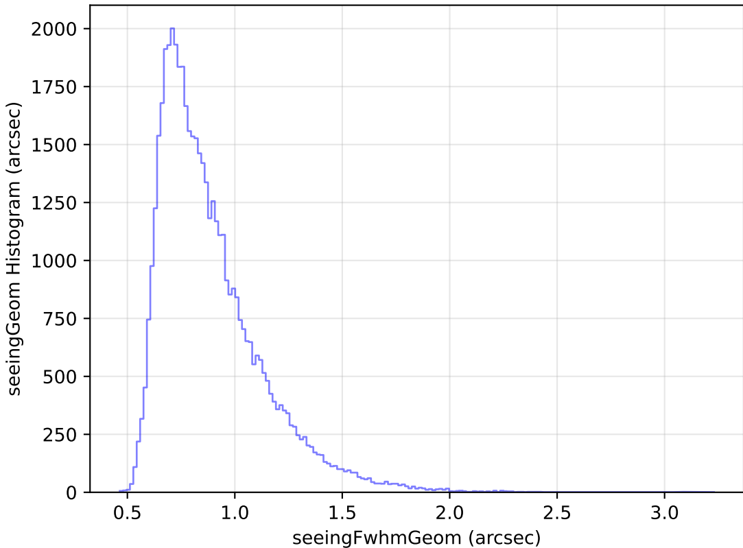
too_elab_r32_d3_giz_v3.4_10yrs Yr 1 r band: seeingGeom Histogram
