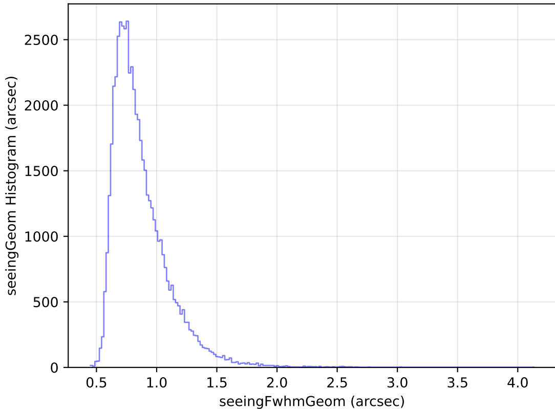
too_elab_r32_d3_giz_v3.4_10yrs Yr 1 i band: seeingGeom Histogram
