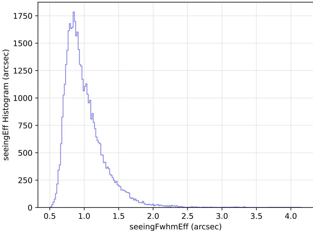
too_elab_r32_d3_giz_v3.4_10yrs Yr 1 z band: seeingEff Histogram
