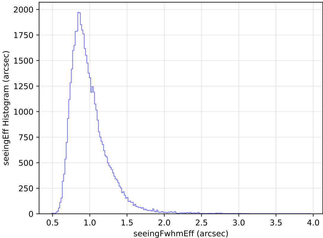
too_elab_r32_d3_giz_v3.4_10yrs Yr 1 y band: seeingEff Histogram
