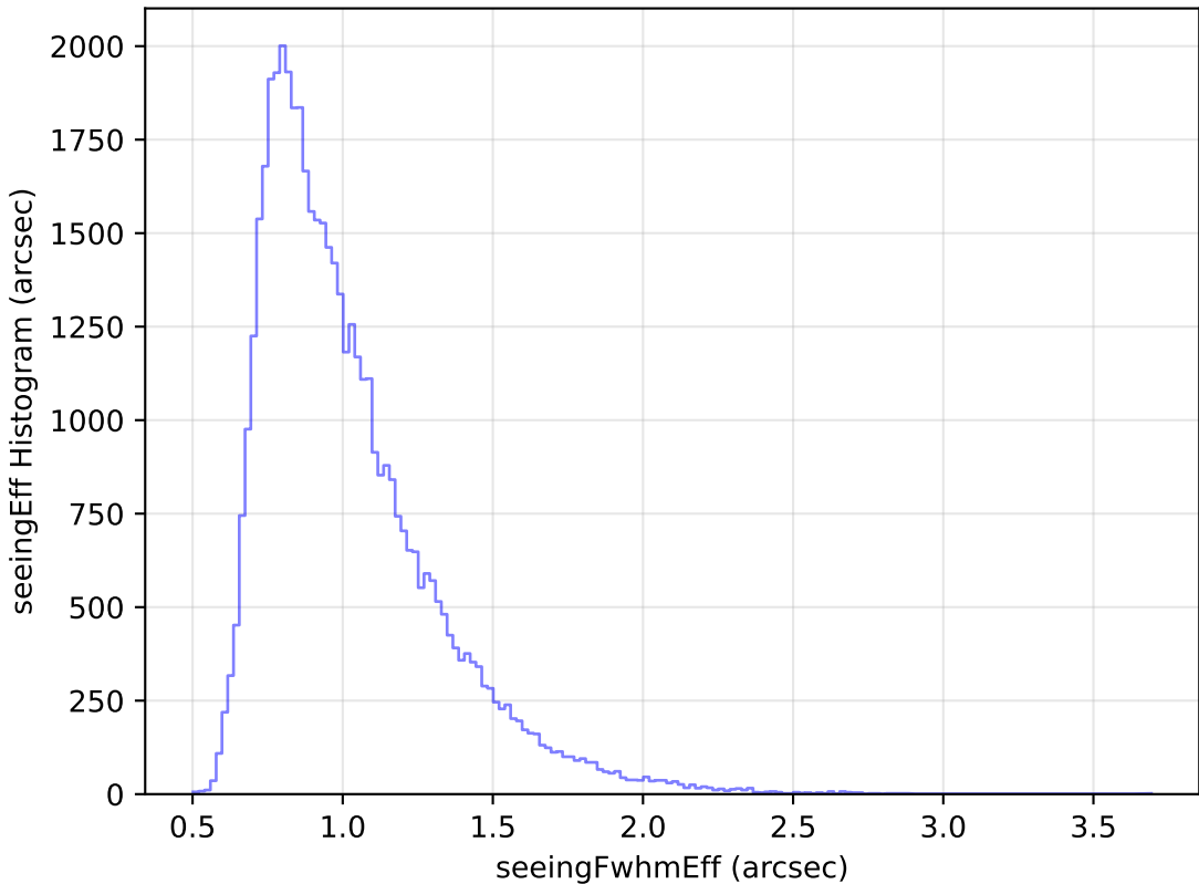
too_elab_r32_d3_giz_v3.4_10yrs Yr 1 r band: seeingEff Histogram
