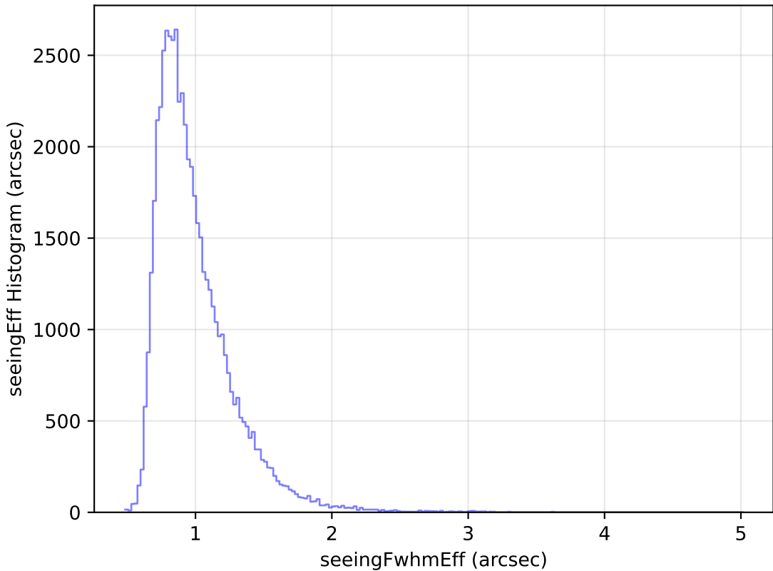
too_elab_r32_d3_giz_v3.4_10yrs Yr 1 i band: seeingEff Histogram
