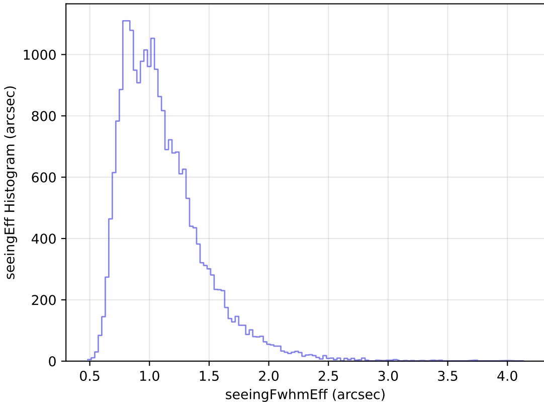
too_elab_r32_d3_giz_v3.4_10yrs Yr 1 g band: seeingEff Histogram
