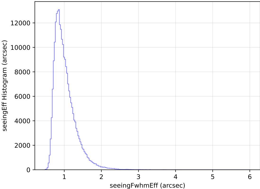
too_elab_r32_d3_giz_v3.4_10yrs Yr 1 all bands: seeingEff Histogram
