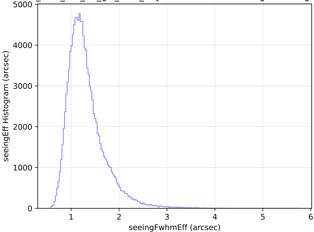
too_elab_r32_d3_giz_v3.4_10yrs WFD u band: seeingEff Histogram
