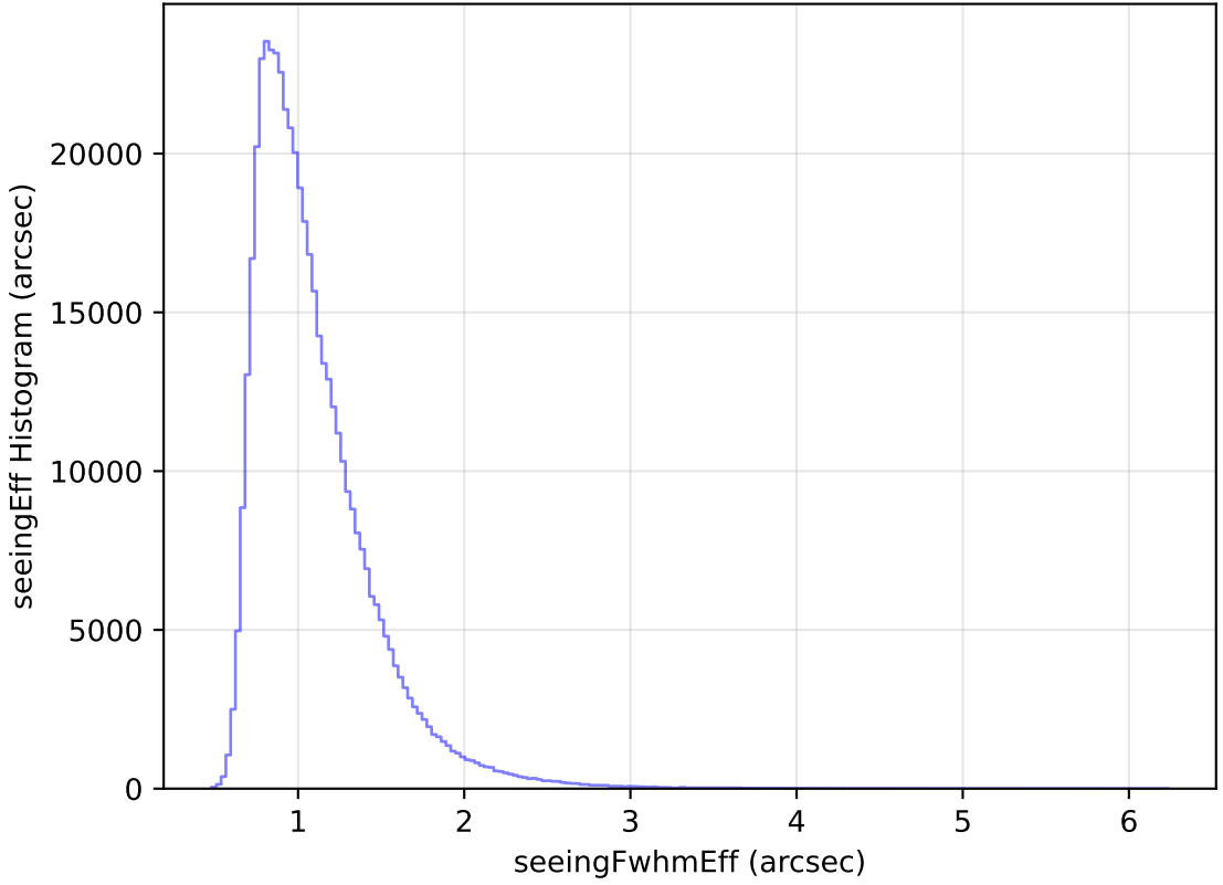
too_elab_r32_d3_giz_v3.4_10yrs WFD i band: seeingEff Histogram
