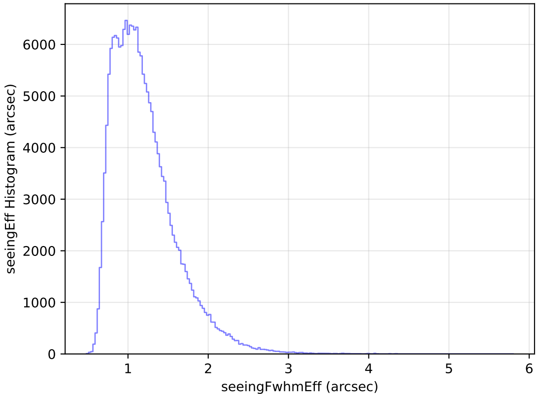
too_elab_r32_d3_giz_v3.4_10yrs WFD g band: seeingEff Histogram
