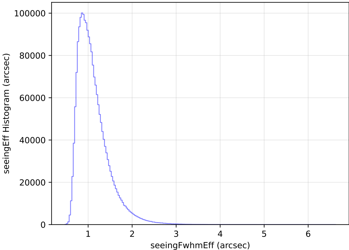
too_elab_r32_d3_giz_v3.4_10yrs WFD all bands: seeingEff Histogram
