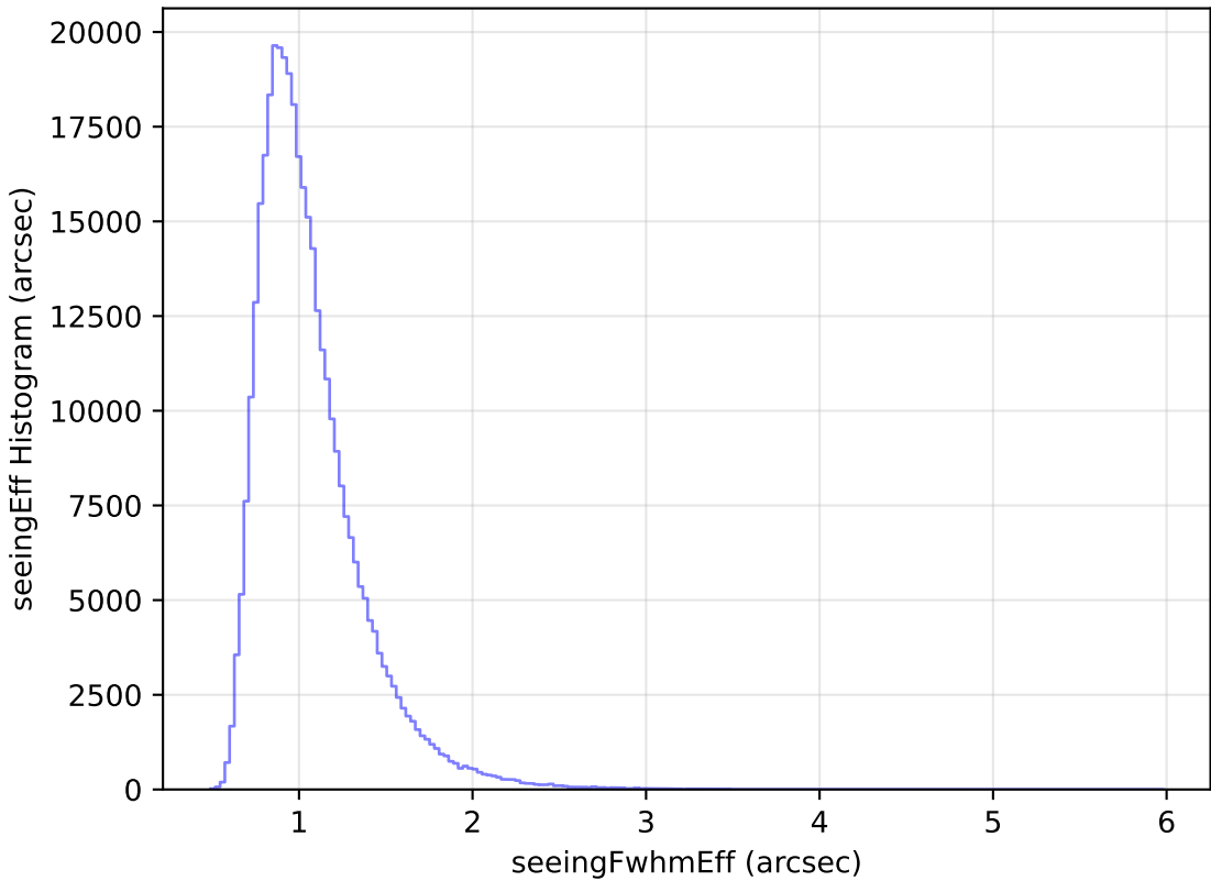
too_elab_r32_d3_giz_v3.4_10yrs All sky y band: seeingEff Histogram
