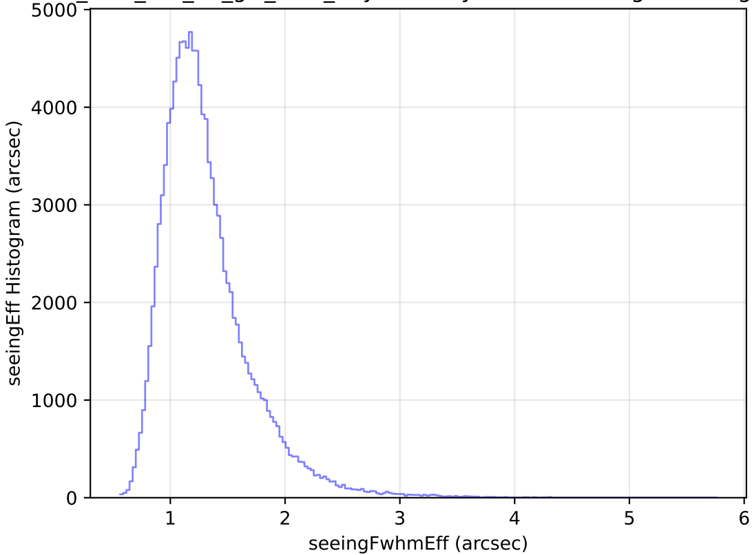
too_elab_r32_d3_giz_v3.4_10yrs All sky u band: seeingEff Histogram
