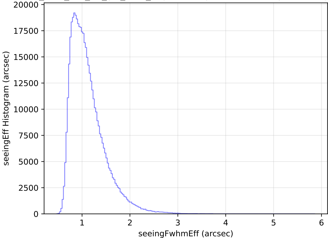
too_elab_r32_d3_giz_v3.4_10yrs All sky r band: seeingEff Histogram
