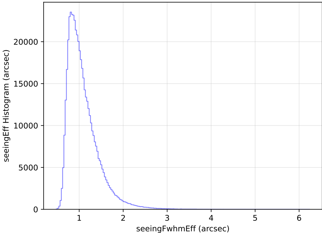
too_elab_r32_d3_giz_v3.4_10yrs All sky i band: seeingEff Histogram
