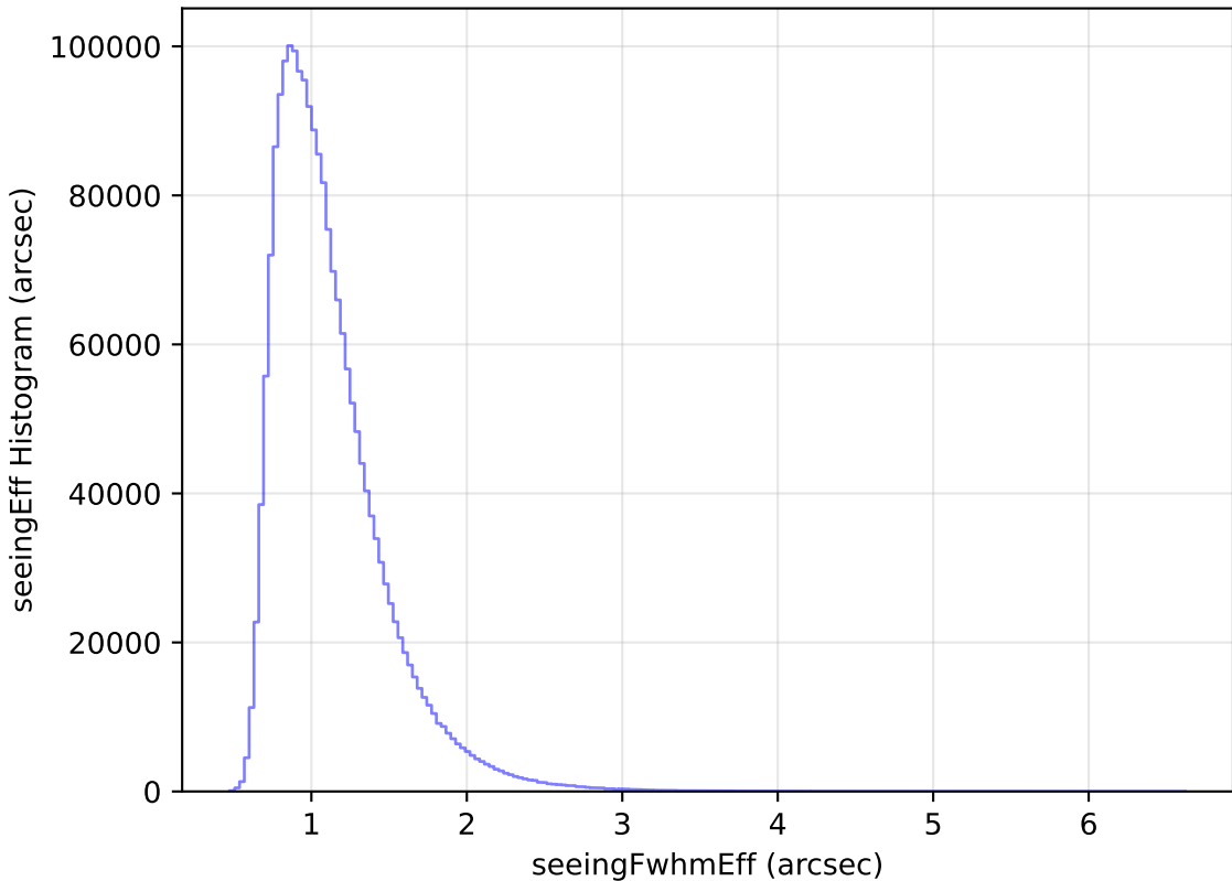
too_elab_r32_d3_giz_v3.4_10yrs All sky all bands: seeingEff Histogram
