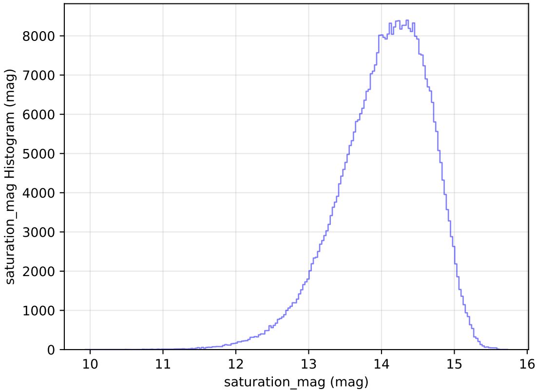
too_elab_r32_d3_giz_v3.4_10yrs WFD z band: saturation_mag Histogram
