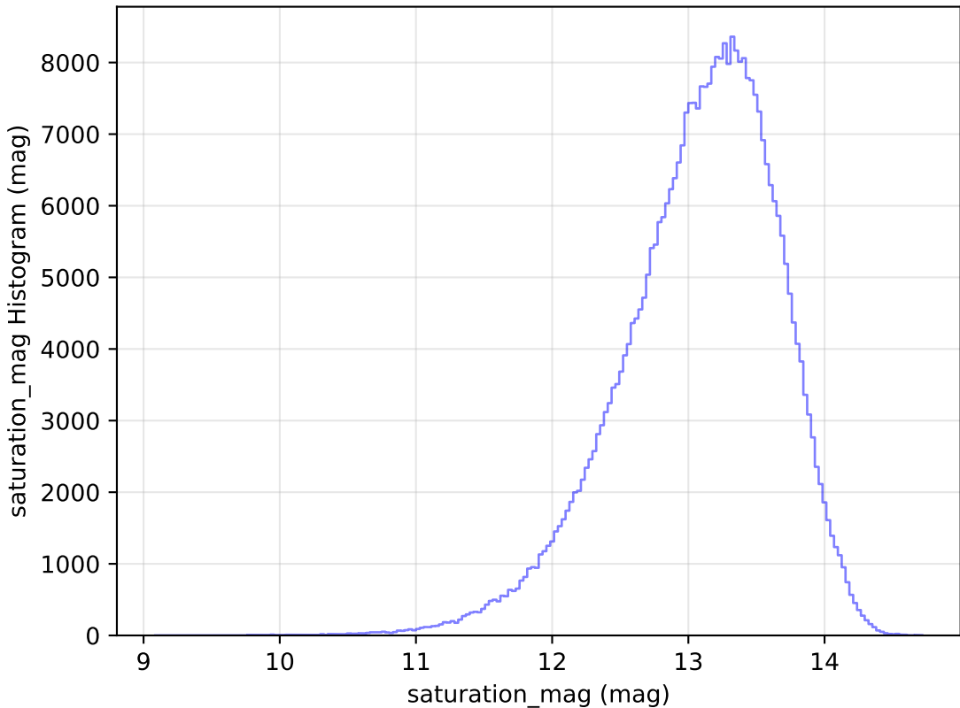
too_elab_r32_d3_giz_v3.4_10yrs WFD y band: saturation_mag Histogram
