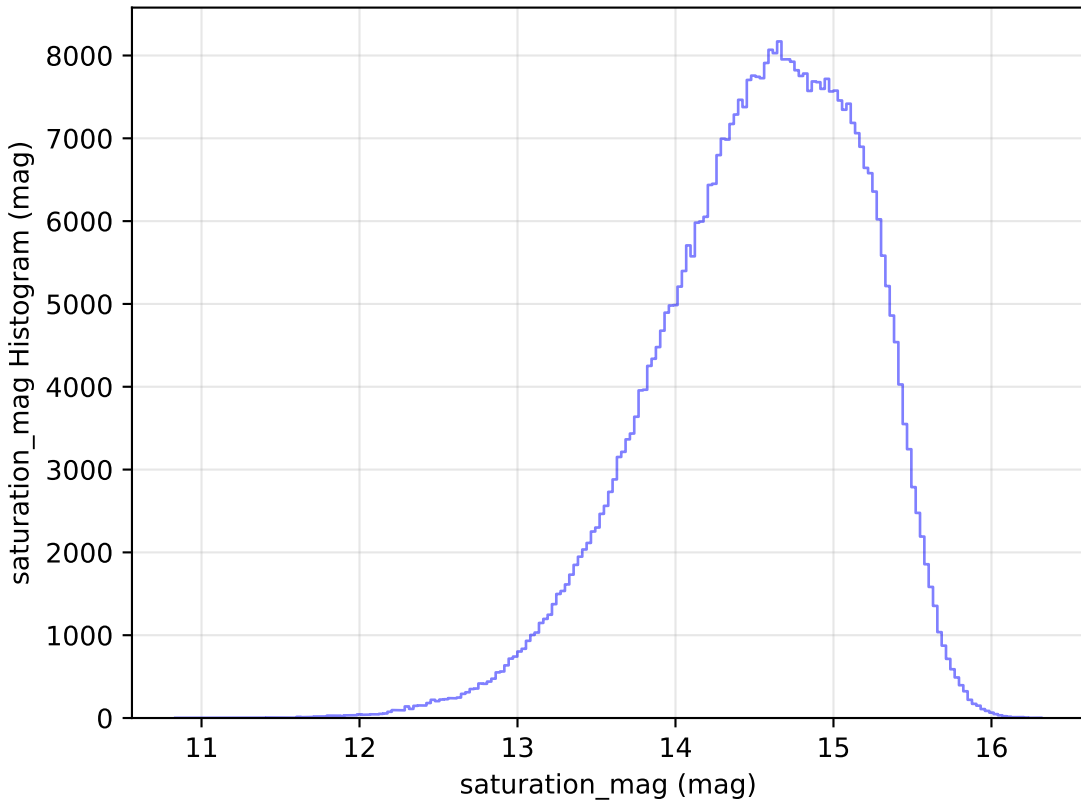
too_elab_r32_d3_giz_v3.4_10yrs WFD r band: saturation_mag Histogram
