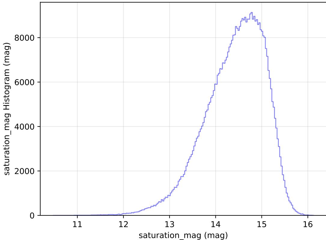
too_elab_r32_d3_giz_v3.4_10yrs WFD i band: saturation_mag Histogram
