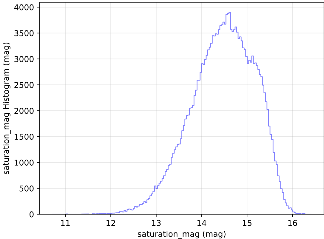
too_elab_r32_d3_giz_v3.4_10yrs WFD g band: saturation_mag Histogram
