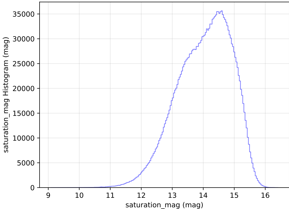
too_elab_r32_d3_giz_v3.4_10yrs WFD all bands: saturation_mag Histogram
