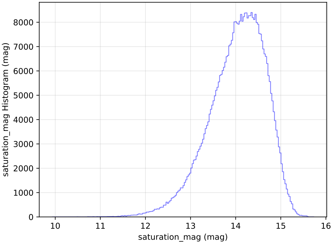
too_elab_r32_d3_giz_v3.4_10yrs All sky z band: saturation_mag Histogram
