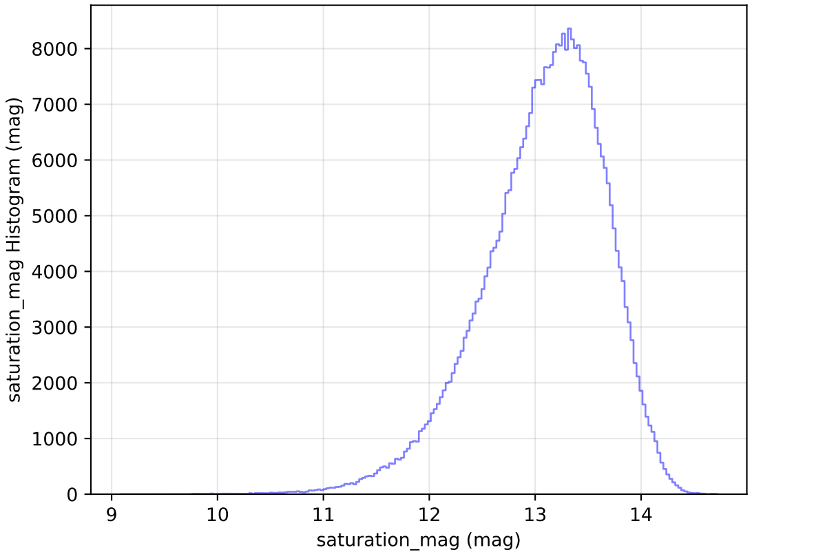
too_elab_r32_d3_giz_v3.4_10yrs All sky y band: saturation_mag Histogram
